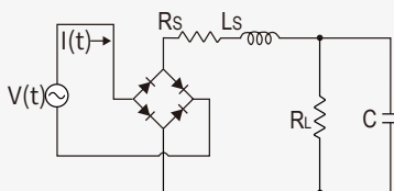
Rectifier single phase rlc
